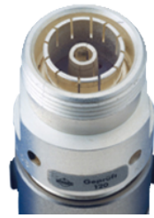
Connector 7-16 socket CAF
