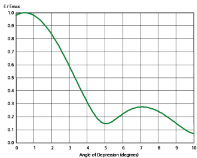
Elevation Pattern - 12 Bay
