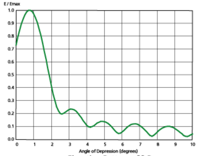
Elevation Pattern - 32 Bay
