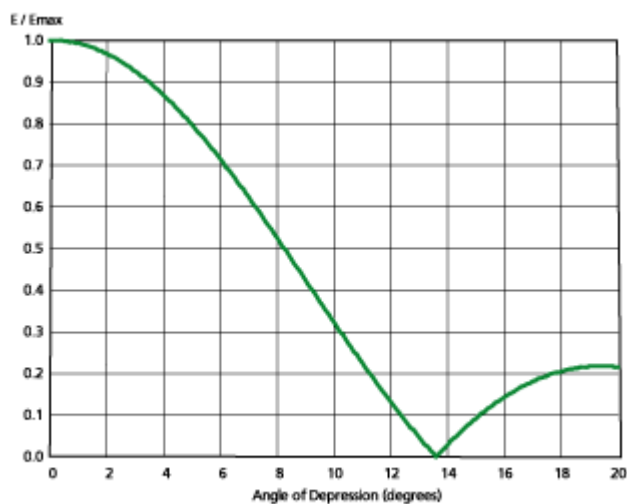
Elevation Pattern - 4 Bay
